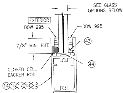
TYPICAL GLAZING DETAIL SCALE: 1/2 FULL
