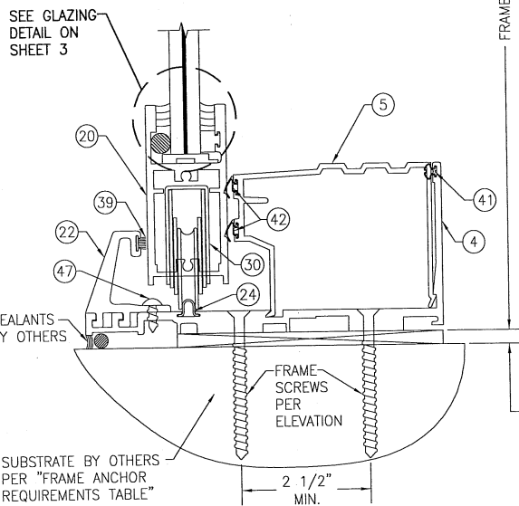
SECTION A SCALE: 1/2 FULL
