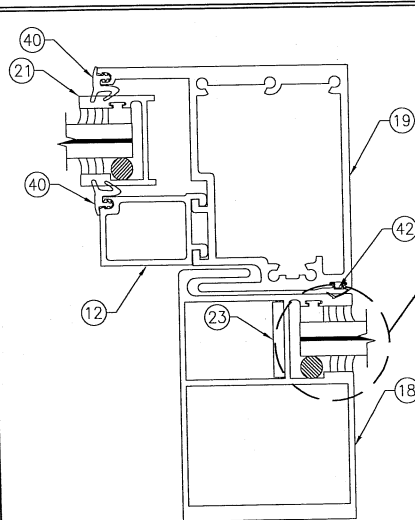
EXTERIOR SECTION SCALE: 1/2 FULL
