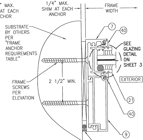
SECTION C SCALE: 1/2 FULL
