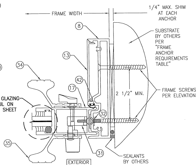
EXTERIOR SECTION SCALE: 1/2 FULL
